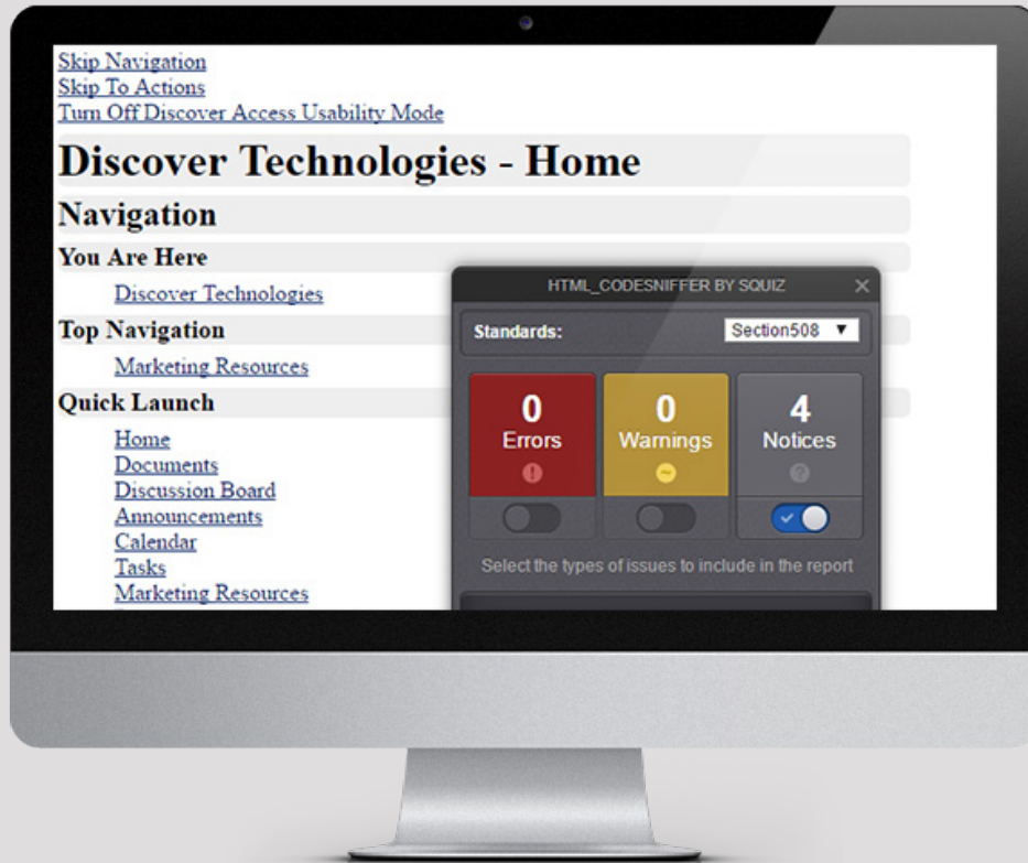
Scan of SharePoint home page with Discover Access Usability Mode turned on
